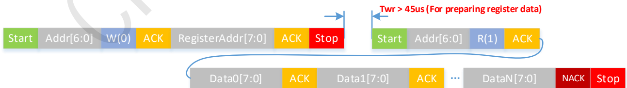
Host Read AXS5106L register
