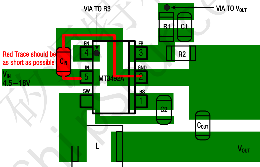
Figure 3. MT3492A Suggested Layout
