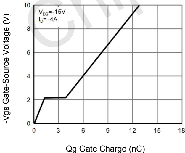
Figure 11 Gate Charge
