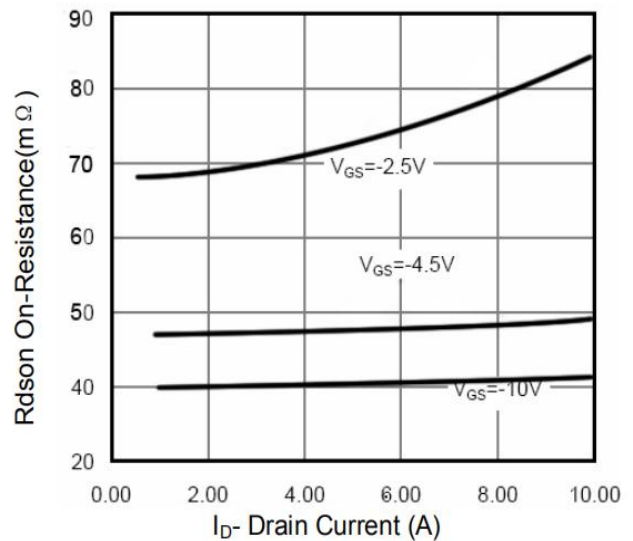
Figure 6 Drain-Source On-Resistance
