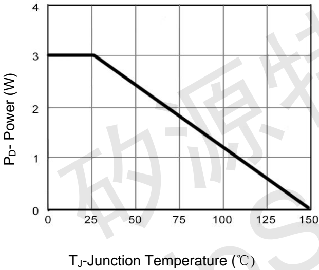
Figure 3 Power De-rating
